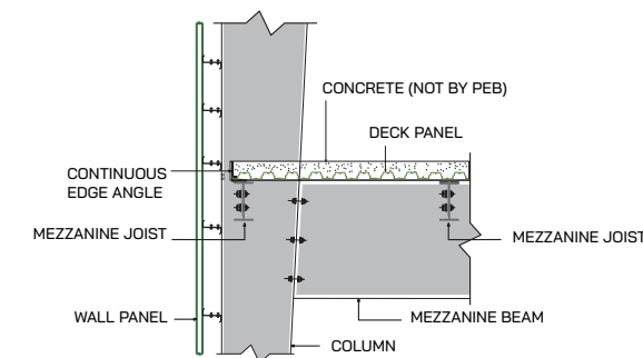
Mezzanine Beam Connection to Main Frame Column
