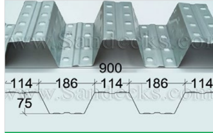
Decking H =75
