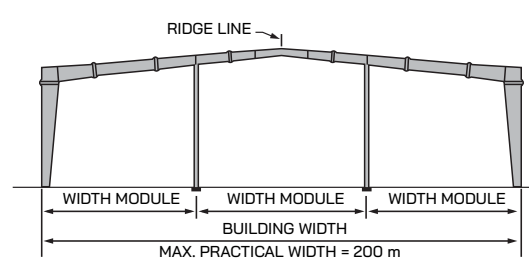
Multi-Span "2" (MS-2)
