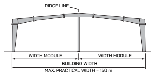
Multi-Span "1" (MS-1)
