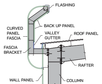
Curved Fascia
