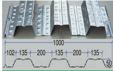
Decking H =50
