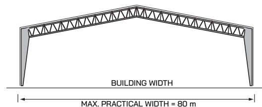
Hybrid
