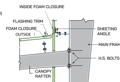
Canopy
