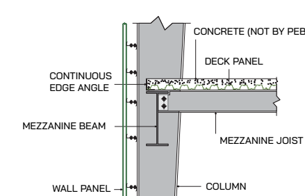
Mezzanine Joist Connection to Mezzanine Beam
