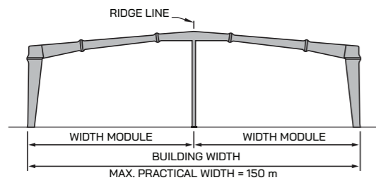
Multi-Span "1" (MS-1)
