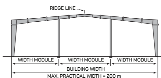
Multi-Span "2" (MS-2)
