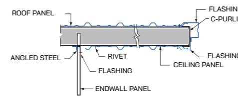
Endwall Roof Extension With Soffit
