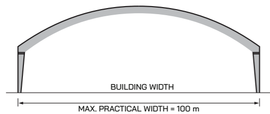
Built-up Curved Rafter (BU)
