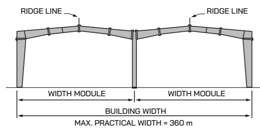
Multi-Gable (MG)
