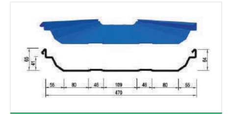
Seamlok Steel Panel
