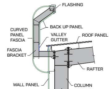
Curved Fascia
